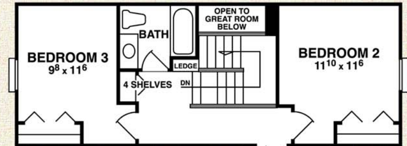
OPTIONAL 2ND FLOOR PLAN ELEV A & B
