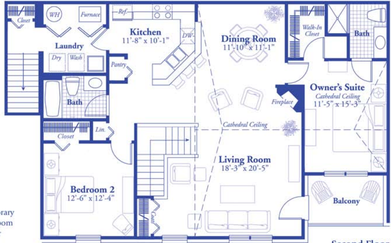
Second Floor
