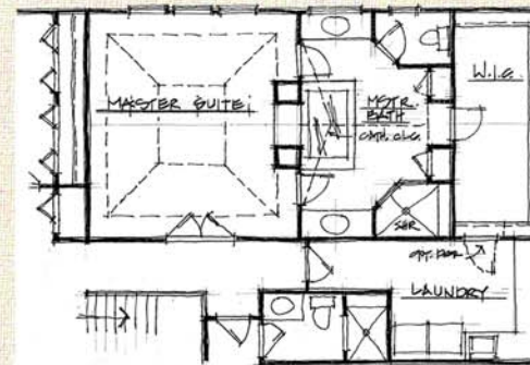
OPT. MASTER BATH WITH DOUBLE SIDED FIREPLACE
