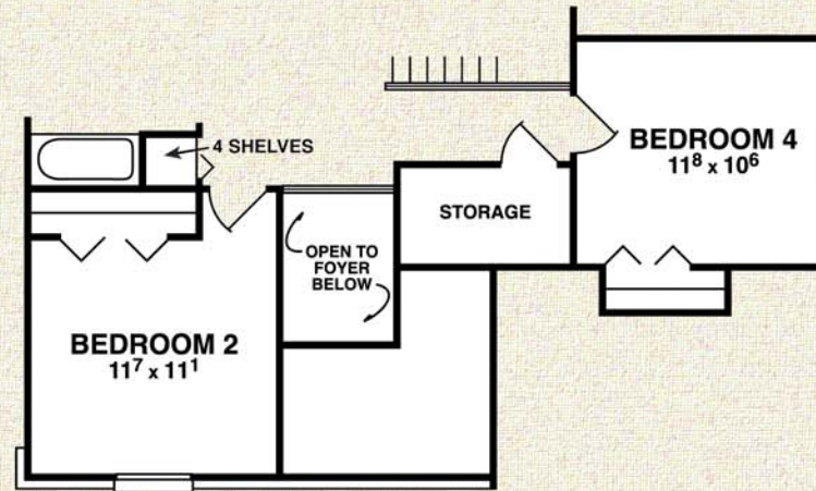
SECOND FLOOR PLAN ELEV B
