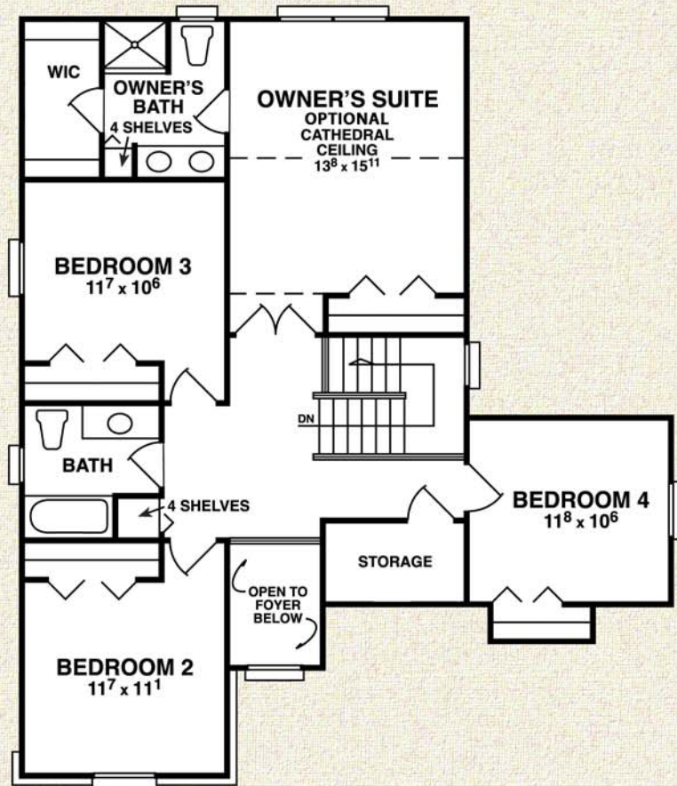
SECOND FLOOR PLAN ELEV C
