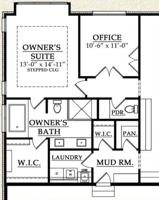
OPTIONAL OWNER SUITE BATH PLAN
